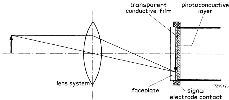
Fig. 2 Target section.
