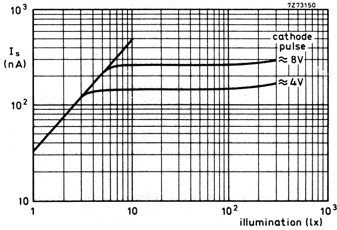
Fig. 2 Typical light transfer characteristics with ACT applied.
