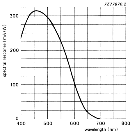
Fig. 3 Typical spectral response for XQ1415.
