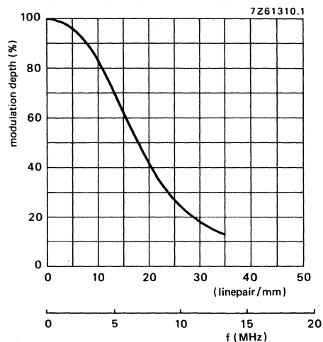
Fig. 2 Typical square-wave response curve.
