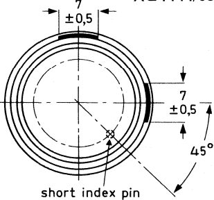
FRONT VIEW XQ ... /15
