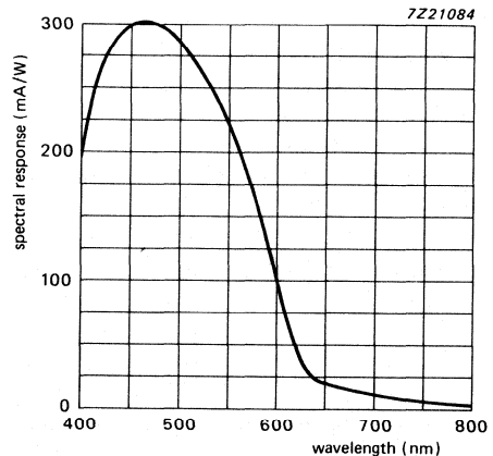
Fig. 2 Typical spectral response for XQ1073R.
