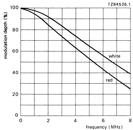
Fig. 5 Typical square-wave response curves for XQ2073-XQ2075.
