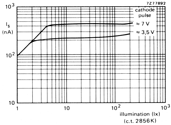
Fig. 2 Typical light transfer characteristics with ACT applied.
