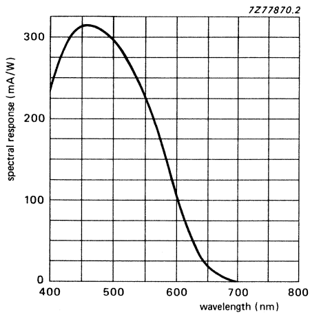
Fig. 5 Typical spectral response for XQ1525R.
