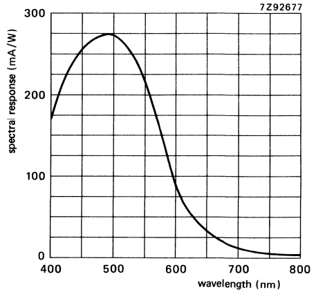
Fig. 2 Typical spectral response.
