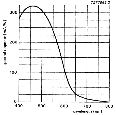
Fig. 2 Typical spectral response for XQ3443R.
