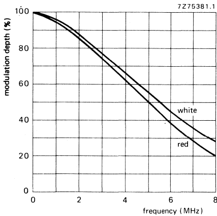
Fig. 6 Typical square-wave response curves for XQ1503R, XQ1505R.
