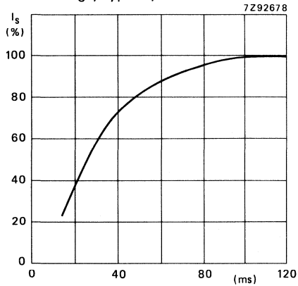
Fig. 3 Build-up lag, I_s/I_b = 100/800 nA without bias light. (Lag can be improved by using bias light).
