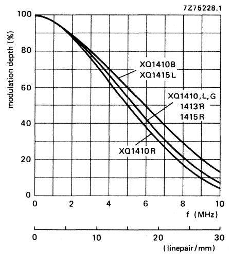
Fig. 4 Typical square wave response curves.
