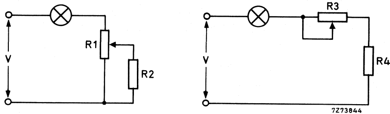
Fig. 7 Supplying the lamp in black/white cameras.
