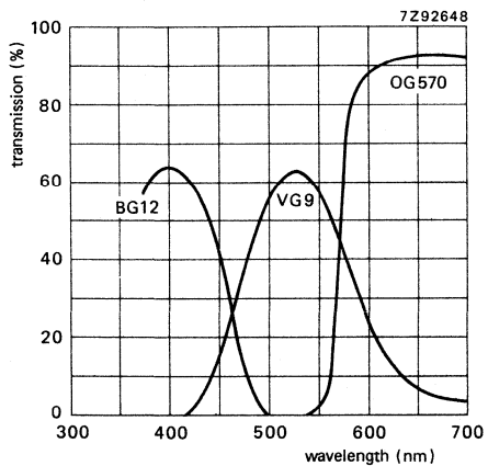
Fig. 4 Transmission of filters BG12, VG9 and OG570.
