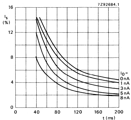
Fig. 6 Decay lag, see note 14. I_s/I_b = 20/300 nA.
