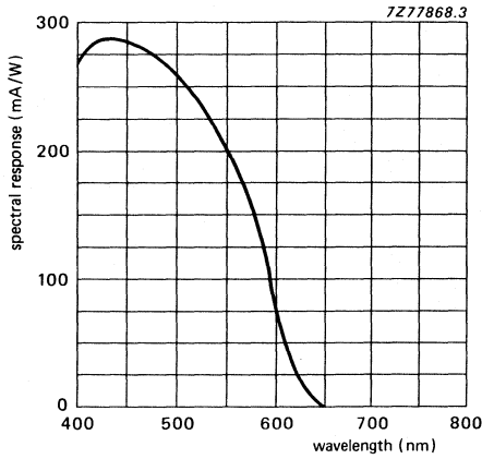
Fig. 1 Typical spectral response for XQ3440, L, R, G, B.
