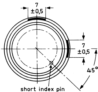
FRONT VIEW 7261433.3 XQ.../12
