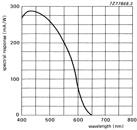
Fig. 1 Typical spectral response for XQ1410.
