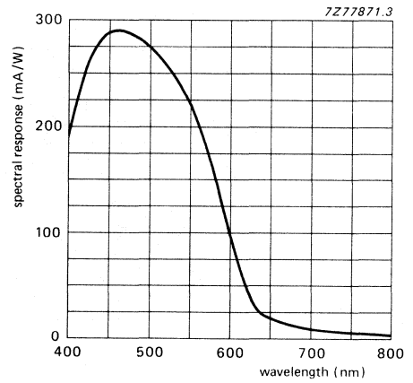
Fig. 4 Typical spectral response for XQ1503R.
