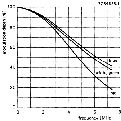
Fig. 4 Typical square-wave response curves for XQ3070
