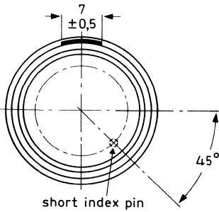
FRONT VIEW XQ ... /05
