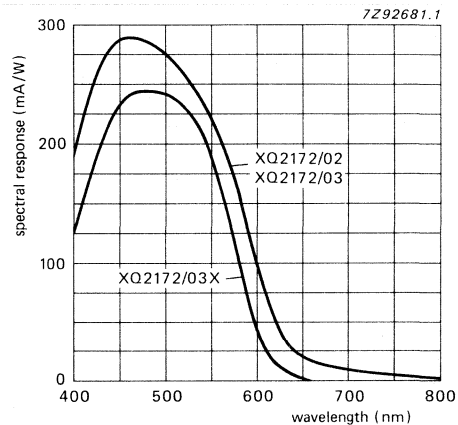
Fig. 4 Typical spectral response curves.
