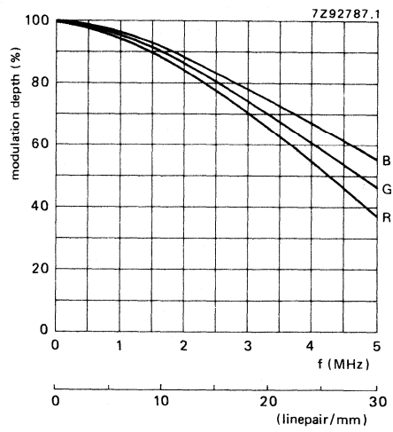
Fig. 2 Typical square wave response curves.
