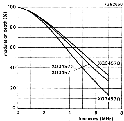
Fig. 6 Typical square-wave response curves.
