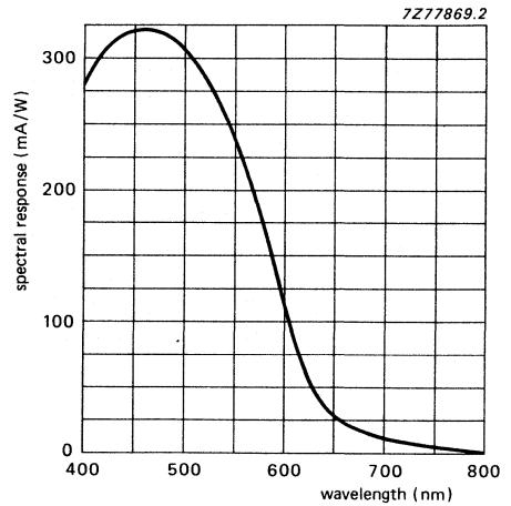
Fig. 4 Typical spectral response for XQ1523R.
