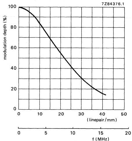
Fig. 2 Typical square-wave response curve.
