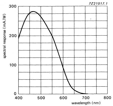
Fig. 3 Typical spectral response for XQ2075R.
