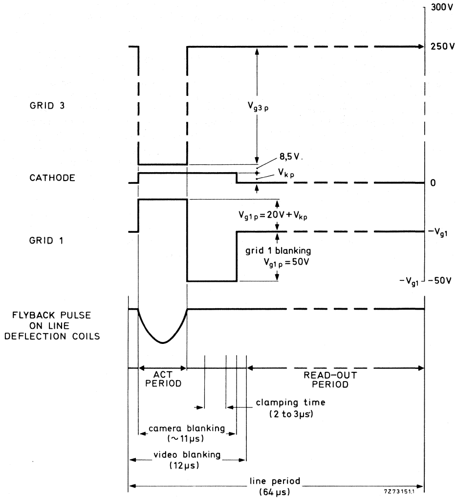
Fig. 1 Pulse timing and amplitude diagram.
