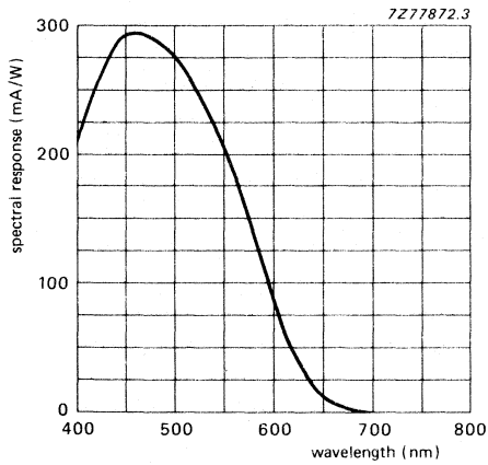
Fig. 3 Typical spectral response for XQ1075R.
