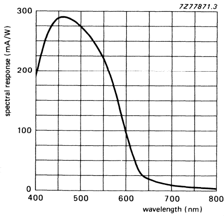
Fig. 2 Typical spectral response for XQ3073R.
