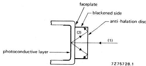
Fig. 9 Anti-halation disc on faceplate.
