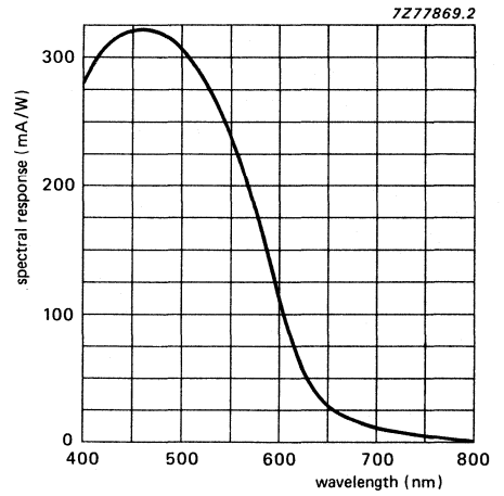
Fig. 2 Typical spectral response for XQ1413.
