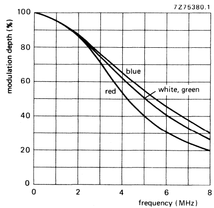
Fig. 6a Typical square-wave response curves for XQ1500.
