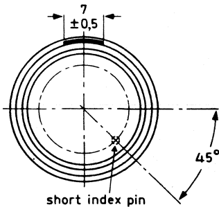
FRONT VIEW 7283927 XQ.../02
