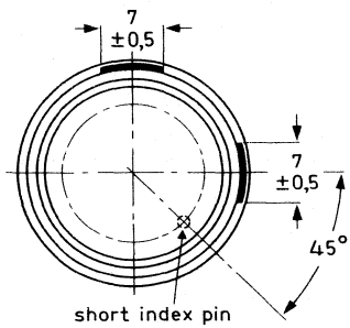
FRONT VIEW XQ2172/02
