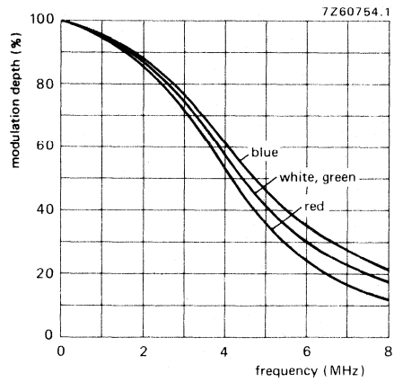
Fig. 4 Typical square-wave response curves for XQ1070.
